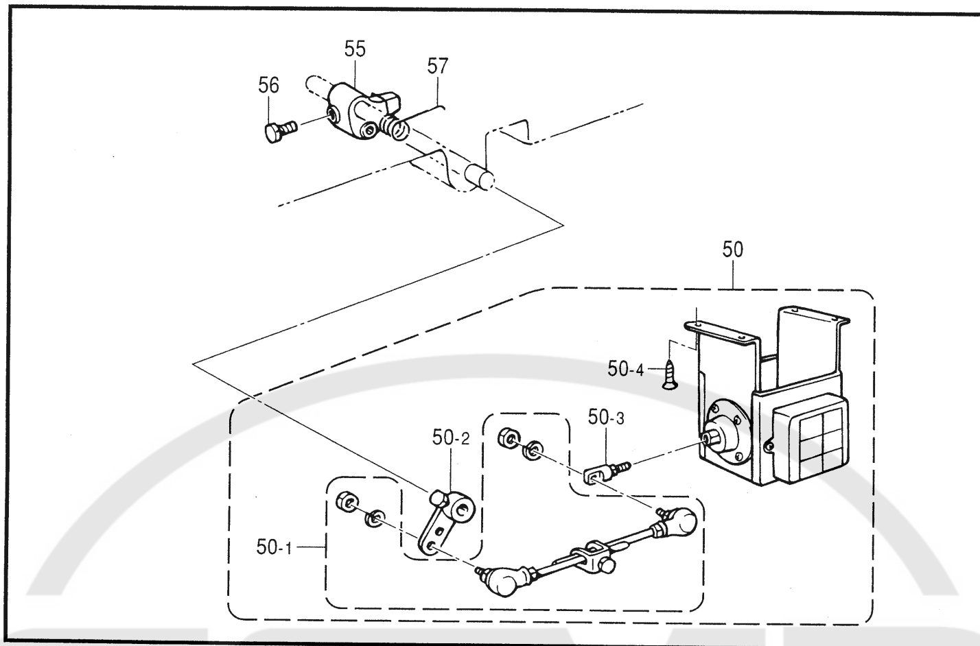
N. 糸暖メ関係 (7220, 7240) / Tension release mechanism (7220, 7240)
